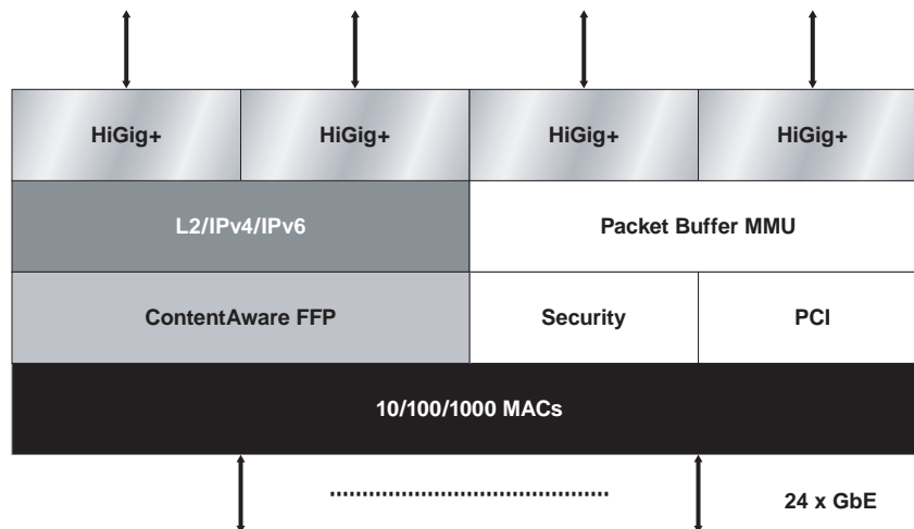
24-Port Gigabit Ethernet Multilayer Switch
